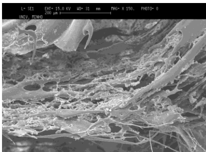
Fig. 3. Micrograph of a location in screw turn 7 showing the the morphology evolution from sheets to droplets (PA6/PP 80/20 wt.%).
