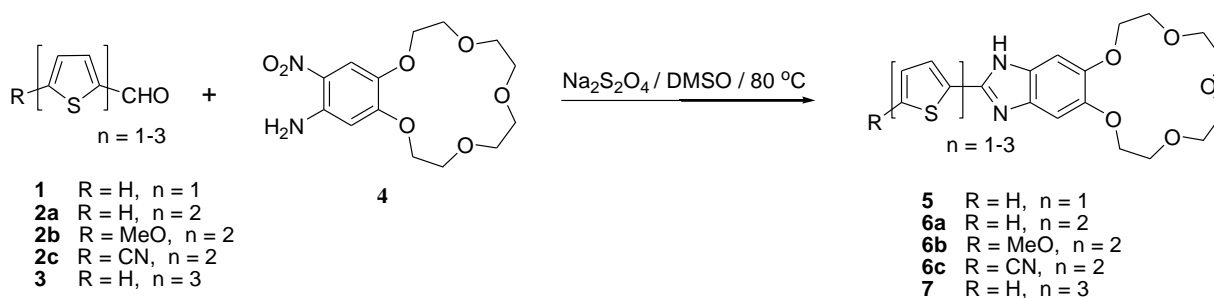
Scheme 1. Synthesis of imidazo[4,5- f ]benzo-15-crown-5 ethers 5-7 .
