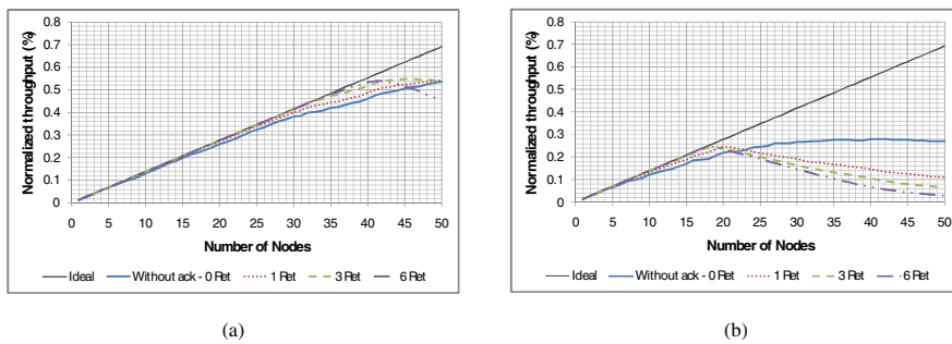
Fig. 6. Normalized throughput curves: (a) star network; and (b) tree network
