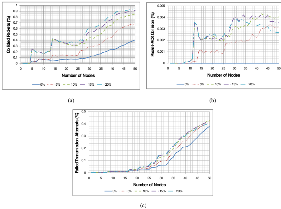
Fig. 13. Hidden-nodes analysis curves: (a) collided packets ratio; (b) packet-ACK collision ratio; and (c) failed transmission attempts ratio
