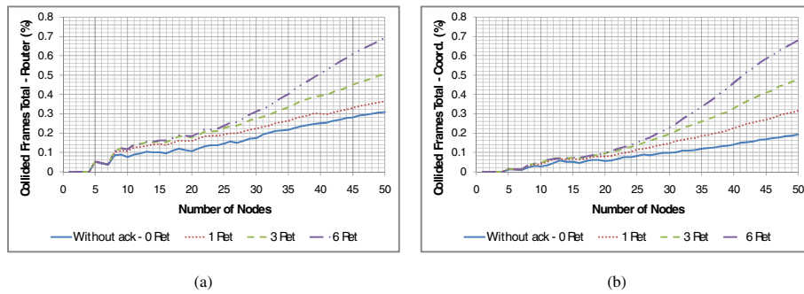
Fig. 4. Tree network packet collision curves: (a) at the router; and (b) at the coordinator
