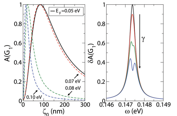
Figure 3: Dependence of the absorption at resonance on the corrugation height (left panel) for different graphene Fermi energies, E_F , and relative absorption for a nonzero metamaterial relaxation's rate \gamma (right panel) with \gamma/\omega_p = \{10^{-4}, 5 \cdot 10^{-4}, 10^{-3}\} (magnitude increasing as indicated by the arrow). (Left panel) The fast change in A(G_1) as E_F varies from 0.07 to 0.08 eV results from a suppression of interband transitions in graphene as 2E_F \gtrsim \hbar\Omega(G_1) . (Right panel) Appearance of two peaks for the highest values of \gamma witnesses a considerable shift of the resonant position of A(G_1) relative to A_{\text{bare}}(G_1) . Other parameters as in Fig. 2.
