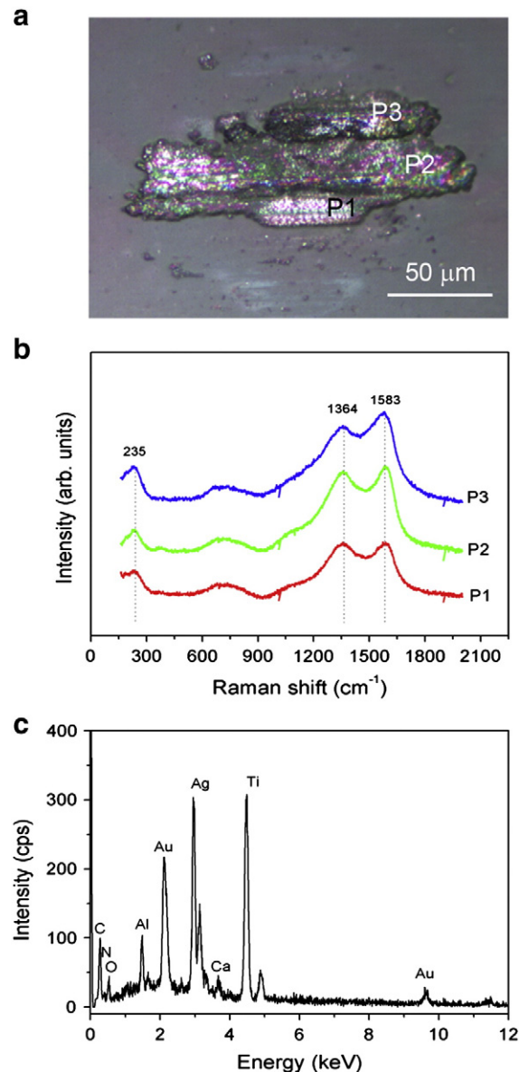
Fig. 8. Optical micrograph of the alumina ball after the friction test onto the Ag-TiCN coating with 10.8 at.% of Ag (a) and corresponding Raman spectra (b) and EDX (c) analysis.
