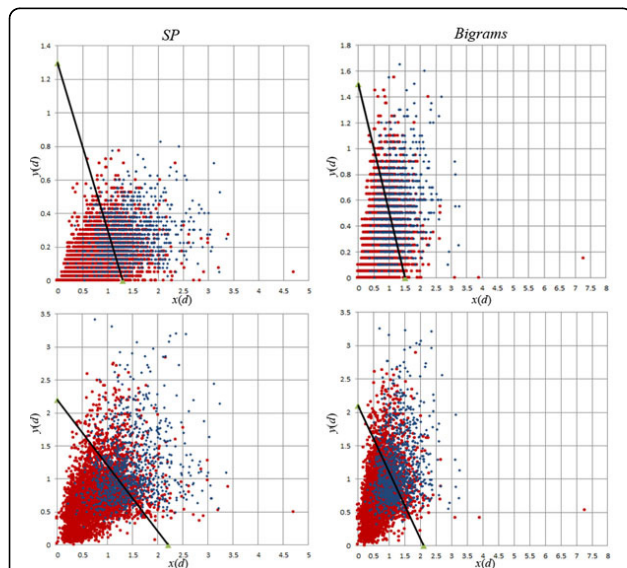
Figure 6 Decision surfaces of the VTT 1 (top) and VTT 5 (bottom) classifiers with SP (left) and bigram (right) features, for the documents in test data. The decision surface and x(d) and y(d) are computed according to Eq. (7) for VTT 1 (top) and Eq. (8) VTT 5 (bottom), for every document d in test set. The plots for VTT 1 surfaces display many documents d with the same values of y(d) , plotted in horizontal rows, while VTT 5 displays a smoother ranking of documents. This happens because VTT 1 uses information from a single NER tool (ABNER protein mentions), while VTT 5 uses information from five such tools; thus, while in the VTT 1 plot many documents have the same value of ABNER protein mentions, in the VTT 5 plot the various NER measurements lead to a finer distinction between documents.
