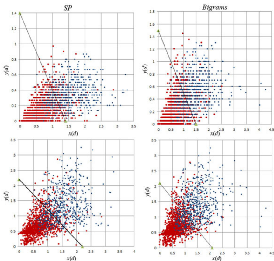
Figure 5 Decision surfaces of the VTT 1 (top) and VTT 5 (bottom) classifiers with SP (left) and bigram (right) textual features, for the documents in one of the validation subsamples of the 4 cross-validation folds using the training data. The decision surfaces are plotted with the parameters in Table 3, and x(d) and y(d) are computed according to Eq. (7) for every document d . The plots for VTT 1 surfaces display many documents d with the same values of y(d) , plotted in horizontal rows, while VTT 5 displays a smoother ranking of documents. This happens because VTT 1 uses information from a single NER tool (ABNER protein mentions), while VTT 5 uses information from five such tools; thus, while in the VTT 1 plot many documents have the same value of ABNER protein mentions, in the VTT 5 plot the various NER measurements lead to a finer distinction between documents.
