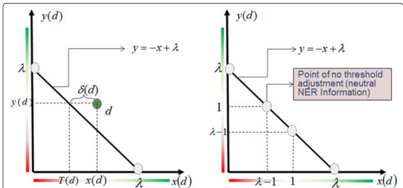
Figure 4 The normalized plane for plotting the VTT decision surface. The coordinates x(d) and y(d) are computed according to Eq. (3) for every document d . The decision surface is computed with Eq. (4). On the left-hand side the threshold for the classification decision is shown (see text for description). On the right-hand side, the point of no threshold adjustment is shown (see text for description).
