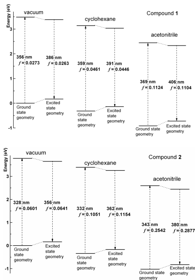
Figure 5. Representation of the energy level diagram, with the transition energies for the benzothienoquinolines 1 (above) and 2 (below), obtained by molecular quantum chemistry calculations, in vacuum, cyclohexane and acetonitrile.
