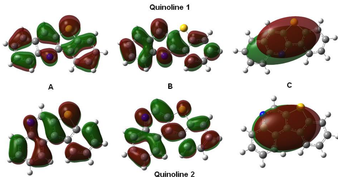
Figure 4. Representation of HOMO orbital (A), LUMO orbital (B) and centroids of charge density depletion ( C_+ , red) or increment ( C_- , green) (C) for compounds 1 and 2 (optimized geometry of the lowest excited singlet state) at an iso level of 0.02 for orbitals and 0.002 for electronic density.
