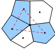
Figure 3: A combination of three cells of \mu(n) are gathered in \mu_k(n) and corresponds to a set of positive barycentric coordinates.
