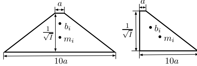
Figure 12: Trapezoidal cells from the hour-glass meshes.
