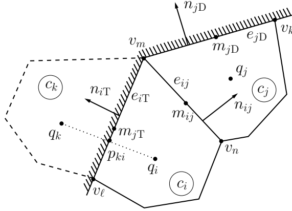
Figure 1: Mesh notation considering real cells (solid lines) and ghost cells (dashed lines).
