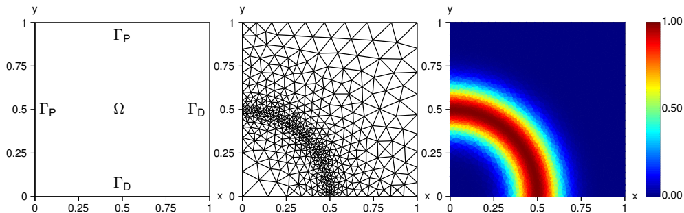
Figure 10: Domain and boundary partitions (left), refined triangular Delaunay mesh (centre), and exact solution with a fine mesh.
