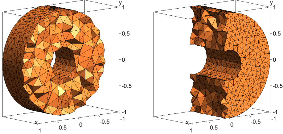
Figure 15: Transversal (left) and longitudinal (right) cross sections of a uniform tetrahedral Delaunay mesh.
