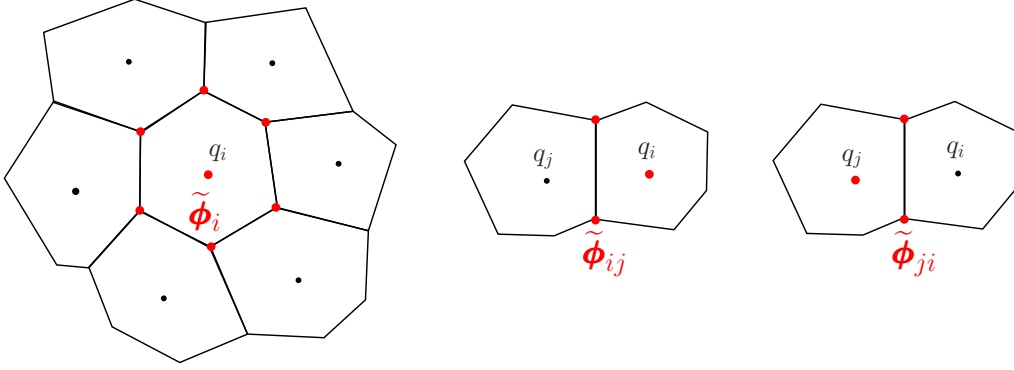
Figure 4: First-degree polynomials for cells (left) and for edges (centre and right). The red dots correspond to the values used in the polynomials reconstructions.
