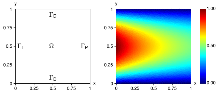
Figure 9: Domain and boundary partitions (left) and the exact solution with a fine mesh (right).
