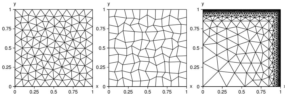
Figure 7: Uniform triangular Delaunay mesh (left), deformed quadrilateral mesh (centre), and locally refined triangular Delaunay mesh (right).
