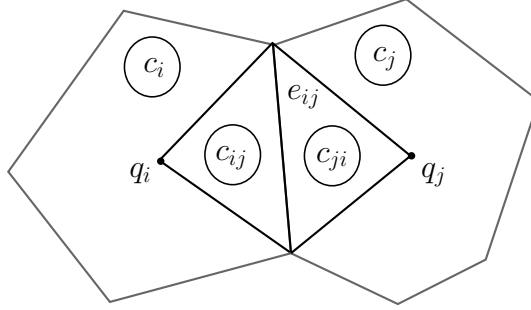
Figure 5: Representation of two subcells, c_{ij} and c_{ji} .
