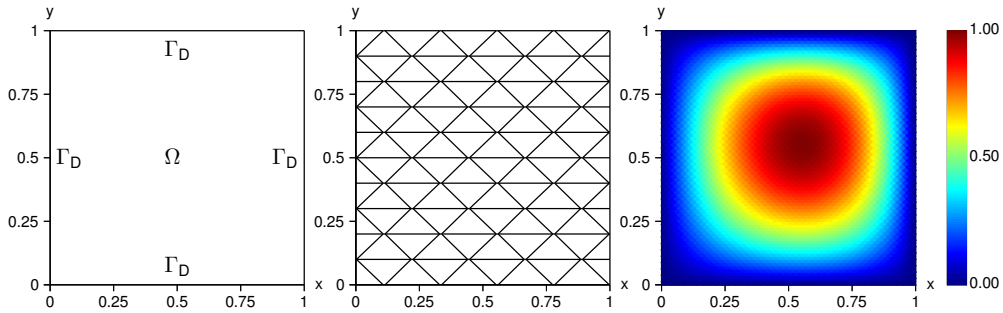
Figure 11: Domain and boundary partitions (left), hour-glass mesh (centre), and exact solution with a fine mesh.
