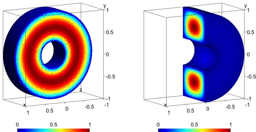
Figure 14: Transversal (left) and longitudinal (right) cross sections of the exact solution with a fine mesh.
