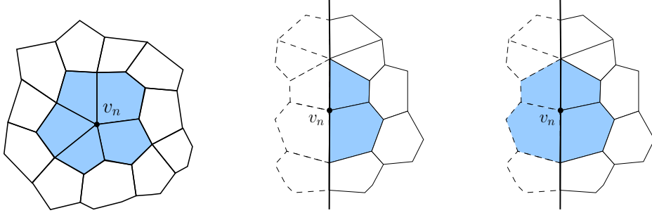
Figure 2: Stencils (colored cells) for the vertices in different situations: \mu(n) = \gamma(n) for an inner vertex (left), \mu(n) for a vertex on \Gamma_T or \Gamma_P (centre), and \gamma(n) for a vertex on \Gamma_T or \Gamma_P (right).
