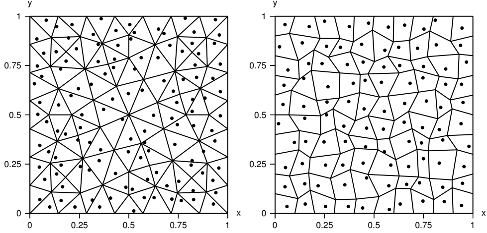
Figure 8: Reference cell points with random locations obtained with \alpha = 0.9 for a triangular Delaunay mesh (left) and a deformed quadrilateral mesh (right).
