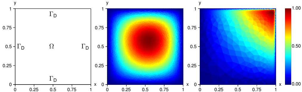
Figure 6: Domain and boundary partitions (left) and exact solutions for the low Péclet number case (centre) and for the large Péclet number case (right) with fine meshes.
