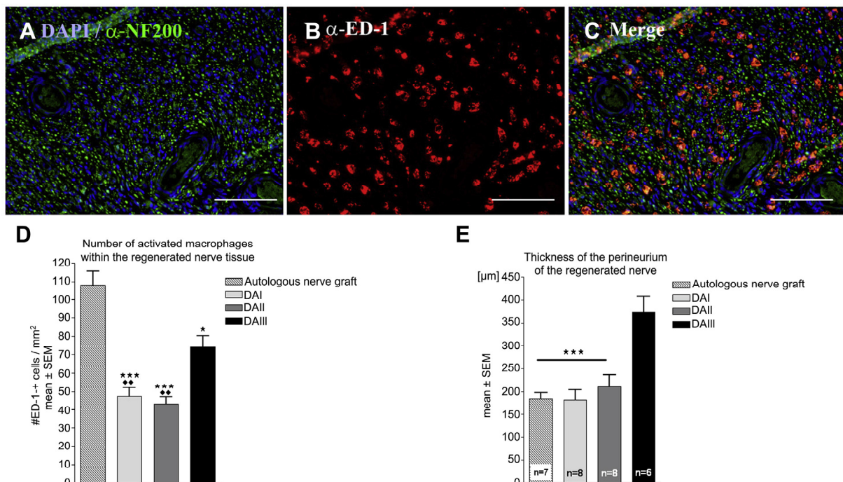
Fig. 10. (A)–(C) Representative photomicrographs of a cross-section of nerve tissue regenerated through DAI/II/III-chitosan tubes analysed for the number of activated macrophages (ED-1-immunopositive cells). (D) Results of ED-1-cell quantification. Significantly less immunological tissue reaction was seen in nerves regenerated through DAI- or DAII-chitosan tubes compared to DAIII-group samples. (E) Measurement of the thickness of the perineurium in the regenerated nerve tissue further revealed that significantly more connective nerve tissue was formed inside of DAIII-chitosan tubes when compared to DAI- and DAII-tubes. DAI = ~2%; DAII = ~5%; DAIII = ~20%. Statistical tests used: (D) Kruskal–Wallis Test, Dunn's multiple comparison, asterisk indicating inter-group differences to autologous nerve graft and solid rhombus indicating inter-group difference to DAIII-chitosan tubes p < 0.05 ; (E) One way ANOVA, Bonferroni multiple comparisons test, asterisk indicating difference to DAIII-chitosan tubes, p < 0.001 .
