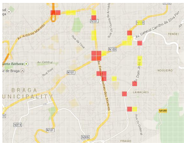
Fig. 4. Region Analysis
