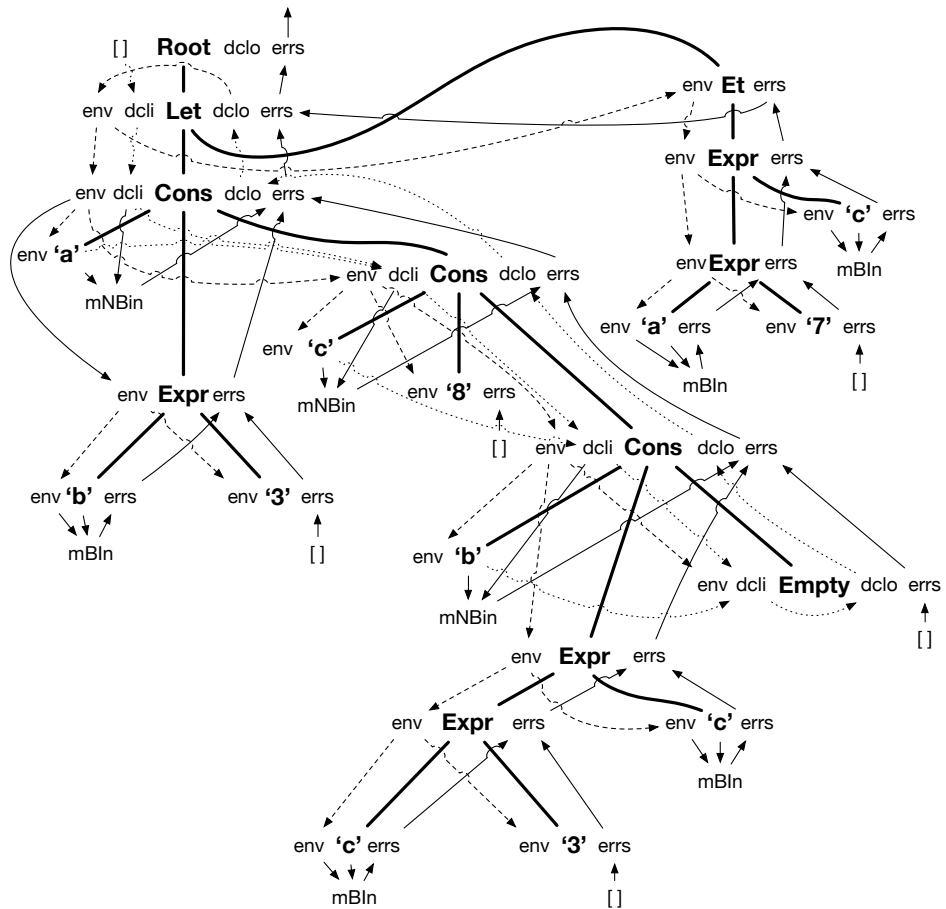
Figure 2.6: The decorated tree for the LET program of Section 2.3. The capture of variables declarations is represented with pointed lines, the distribution of variables with dashed lines and the calculation of identifiers with black lines.
