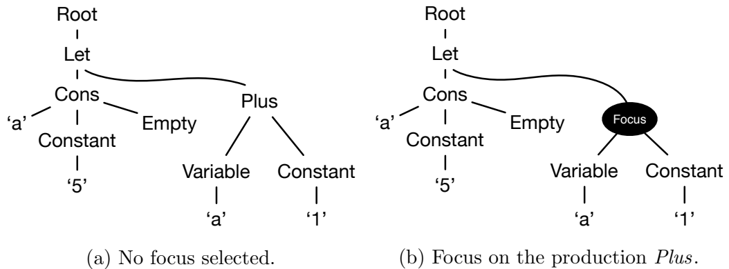
Figure 3.3: Tree representation of zipper_example .
