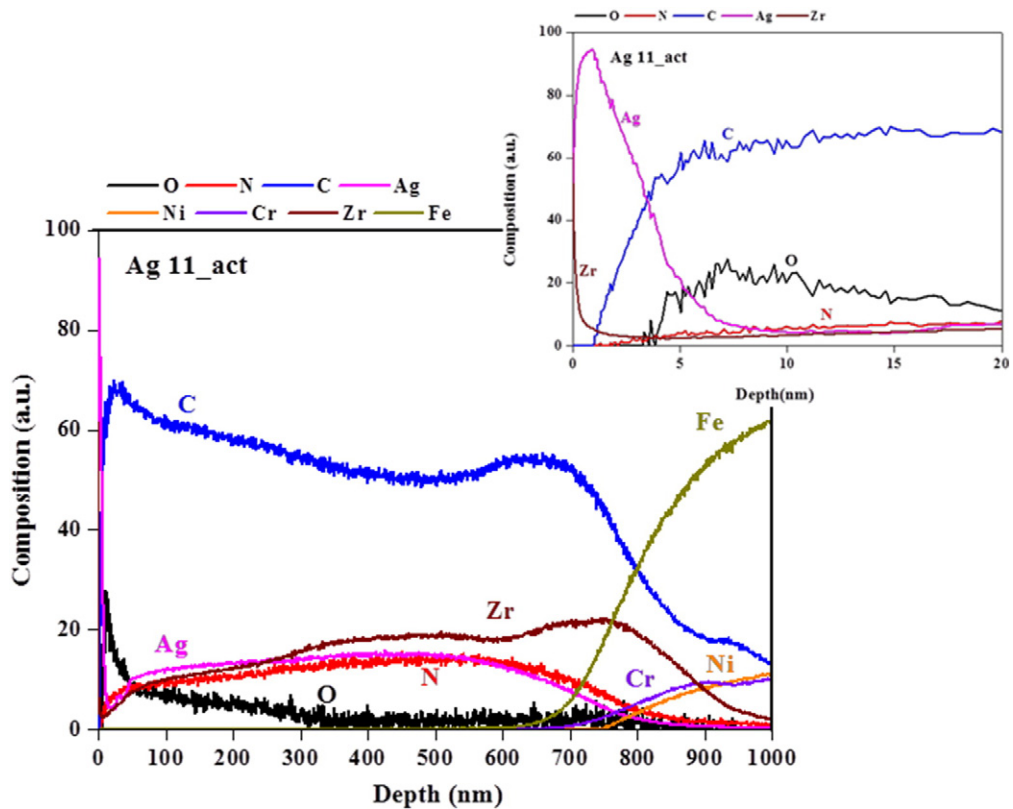
Fig. 4. GDOES profile of Ag 11 thin film after activation with NaClO. The inset in the figure shows the profile in the first 20 nm of the coating.
