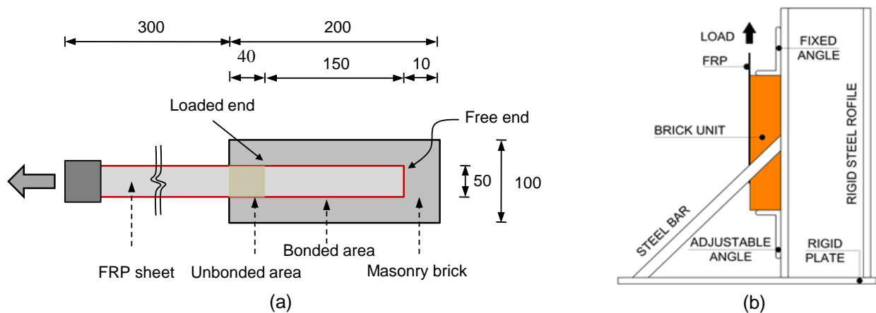
Figure 2. Shear bond tests (single-lap shear bond): (a) geometry of the specimens (dimensions in mm); (b) scheme of the test setup.
