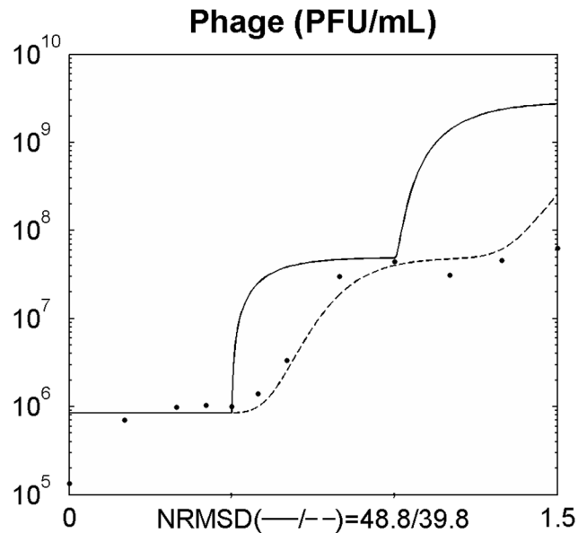
Fig 1. Simulating the one step growth curve using a normal distribution function (equations 6–14).
