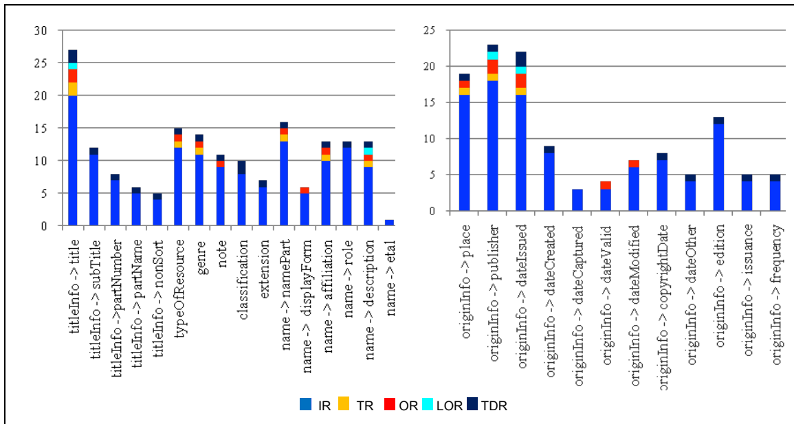
FIG. 5. MODS elements and subelements used by Digital Repository (titleInfo, typeOfResource, genre, note, classification, extension, name, originInfo Elements)
