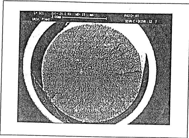
Figure 6. SEM micrograph of a tensile fracture surface of a SCORIM-S2-molded 5-mm SEVA-C/30%-HA composite.
