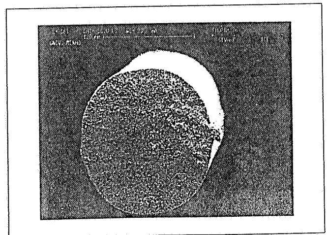
Figure 5. SEM micrograph of a tensile fracture surface of a conventionally molded 1.5-mm SEVA-C/30%-HA composite.
