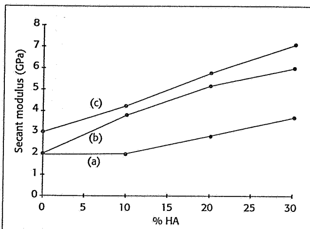
Figure 1. Modulus versus % HA for the following processing methodologies: (a) RD/conventional, (b) TSE/conventional, and (c) TSE/SCORIM.
