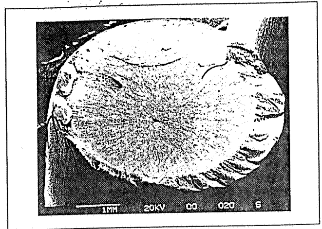
Figure 3. SEM micrograph of a tensile fracture surface of a conventionally molded 5-mm SEVA-C sample.
