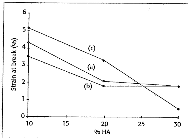
Figure 2. Strain at break versus % HA for the following processing methodologies: (a) RD/conventional, (b) TSE/conventional, and (c) TSE/SCORIM.
