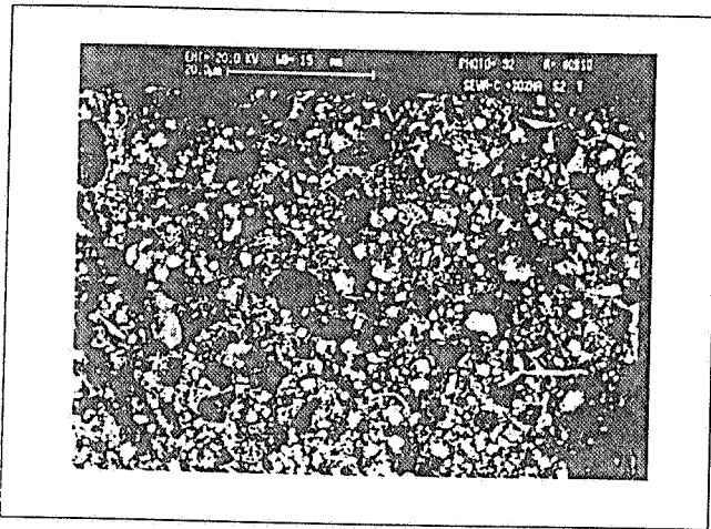
Figure 7. Superimposed secondary and back-scattered electron images showing the HA distribution in a SEVA-C/30%-HA composite.
