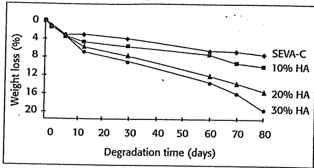
Figure 8. Dry weight loss versus degradation time in HBSS at 37°C for SEVA-C and several HA-reinforced composites.
