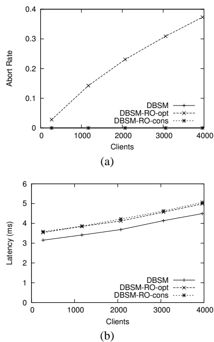
Figure 2: Performance of read-only transactions.
