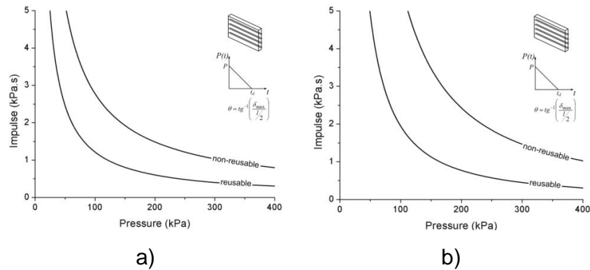
Figure 10. P-I diagram for masonry infill panel with minimum bed joint reinforcement: a) 180 mm; b) 230 mm.
