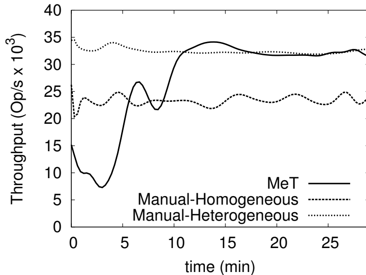
Figure 3.4: Evaluation results
