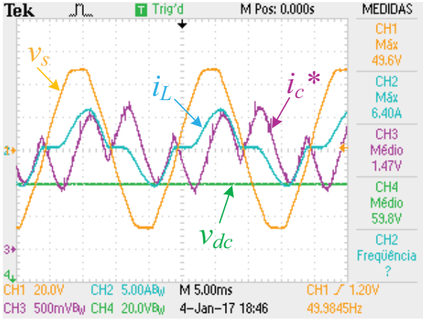
Fig. 3. Experimental results during the operation as active power filter: Power grid voltage ( v_s ); Load current ( i_L ); Dc-link voltage ( v_{dc} ); Converter current reference ( i_c^* ).
