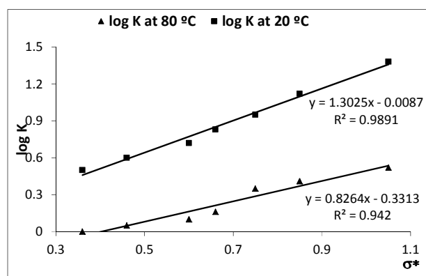
Scheme 1 Plot of log K ( K = [\mathbf{5}]/[\mathbf{2}] ) in DMSO- d_6 versus the Hammett-Brown parameters \sigma^* .
