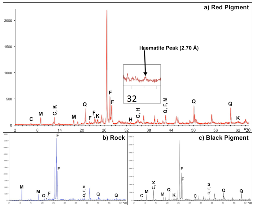
Figure 6. XRD analysis of the Leandro 5 mound pigments: (a) red pigment, (b) rock from an undecorated area and (c) black pigment. The identified mineral phases were as follows: C, clinocllore; K, kaolinite; H, haematite; Q, quartz; M, micas; F, feldspars.
