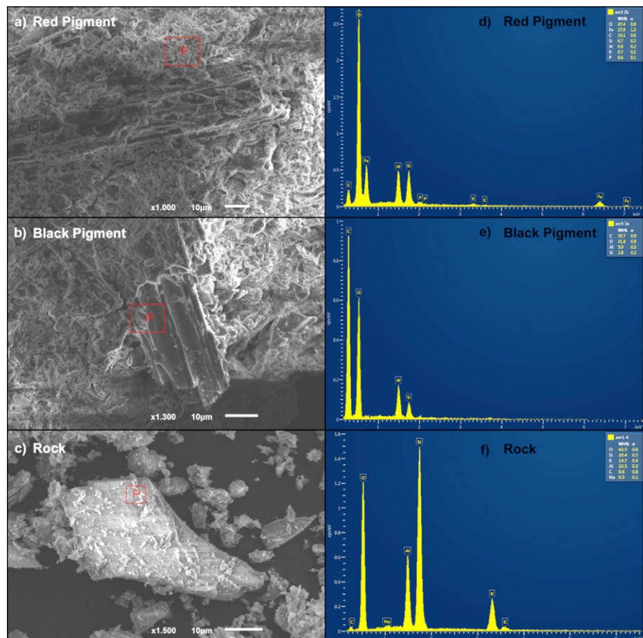
Figure 7. SEM images from the (a) red pigment, (b) black pigment and (c) undecorated rock. EDS spectra from the (d) red pigment, (e) black pigment and (f) undecorated rock.
