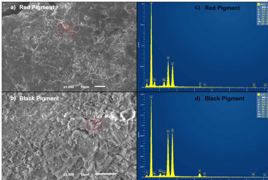
Figure 8. Analysis of the Leandro 5 mound pigments. SEM images (a and b) and EDS spectra (c and d) from the black and red pigment. In the EDS spectra it is possible to observe the presence of Mg.
