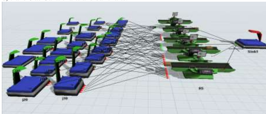
Figure 3. Snapshot of the FlexSim Simulation setup.
