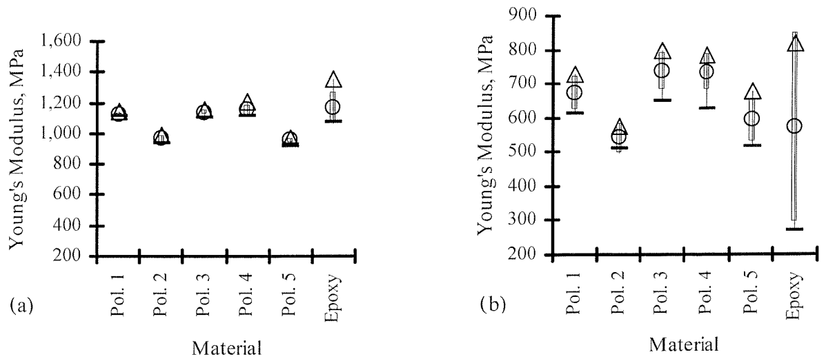
Fig. 4. Young's modulus determined at (a) 20 and (b) 40°C.
