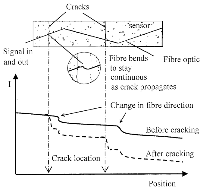
Fig. 1. Principle of operation of “zigzag” sensor.
