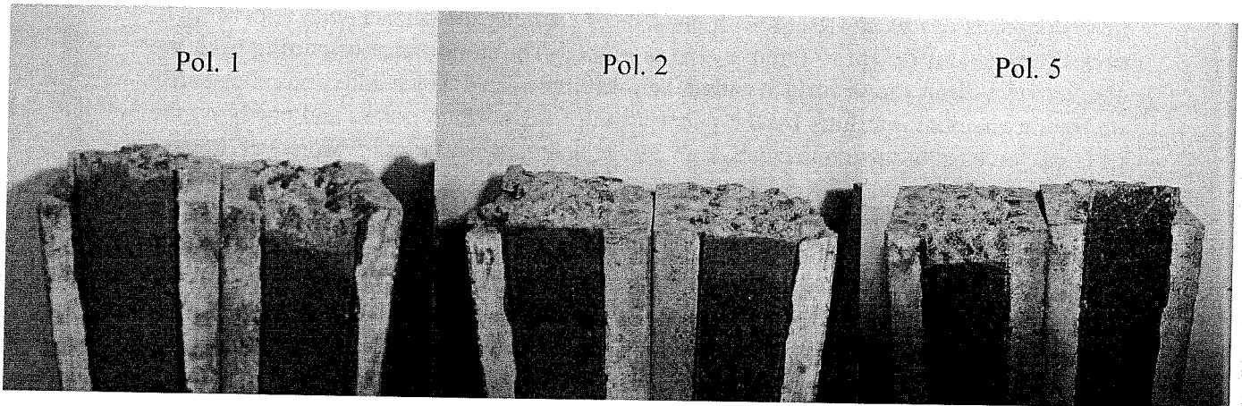
Fig. 13. Specimens after failure.
