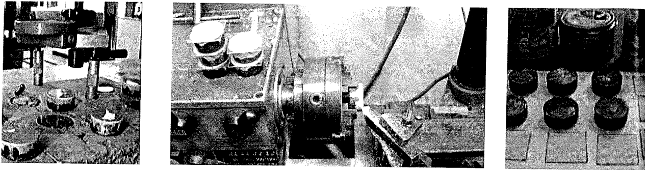
Fig. 16. DYNA, T. F. 16 kN, specimen preparation and rectification in pull-off tests.
