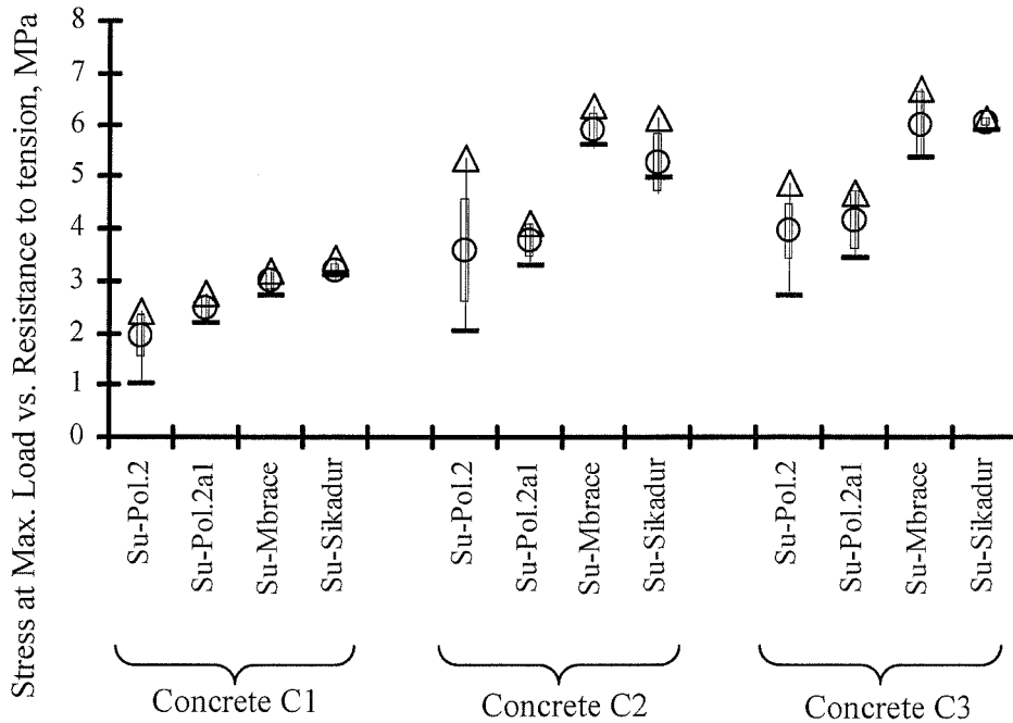
Fig. 15. Pull-off stress of adhesion/tensile strength.
