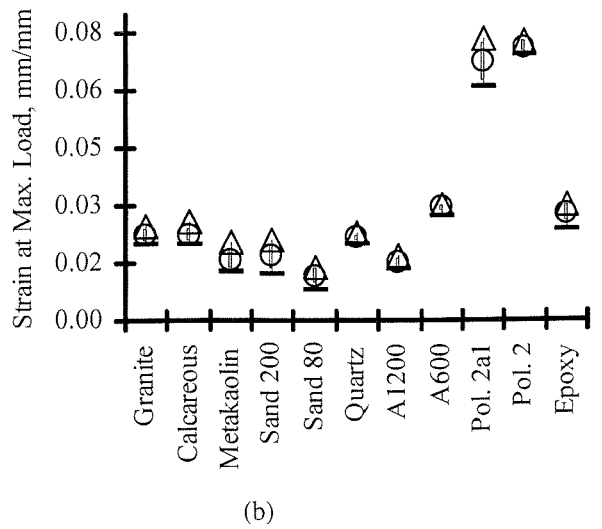
Fig. 10. Tensile strain at maximum load at 20°C of Pol. 2a1 with different additions: (a) 10% of addition material, (b) 20% of addition material.
