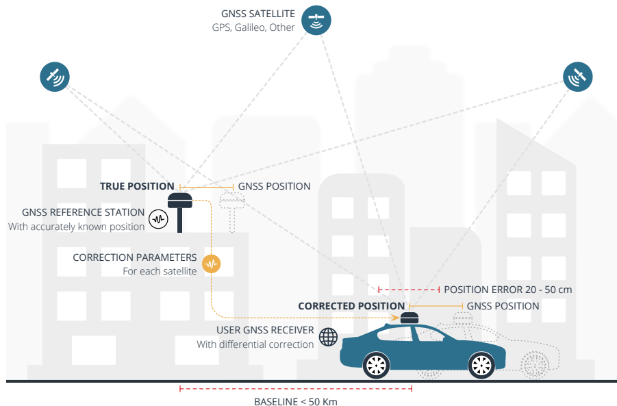
Figure 3: Classic Differential GNSS (DGNS)
