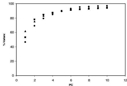
Figure 3. Percentage captured variance for each PC in the PCA model of mean centred spectra of samples collected from the feed (●), the reactor (■) and the settler (▲).
