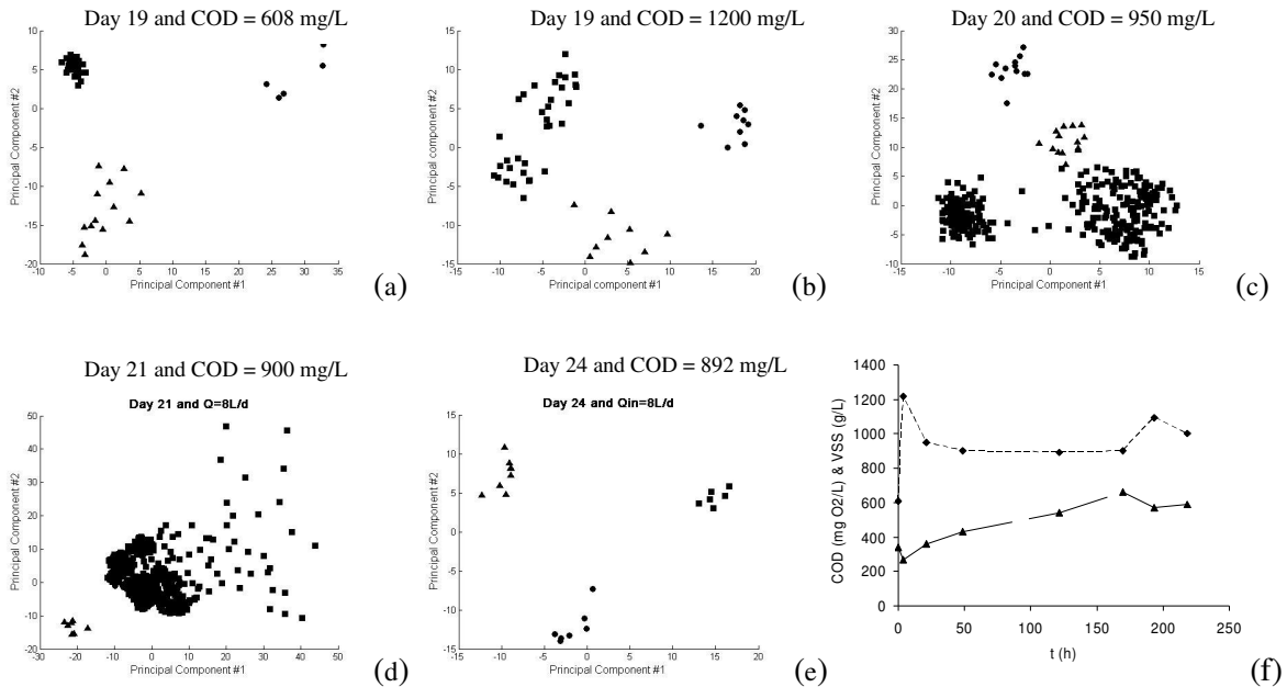
Figure 6. Evolution of the state of an aerobic biological reactor monitored through the analysis of score plots including the three monitored points of the reactor: Feed (●), Reactor (■) and Settler (▲). Figure (f) represents the evolution of the COD in the feed and the VSS in the reactor.
