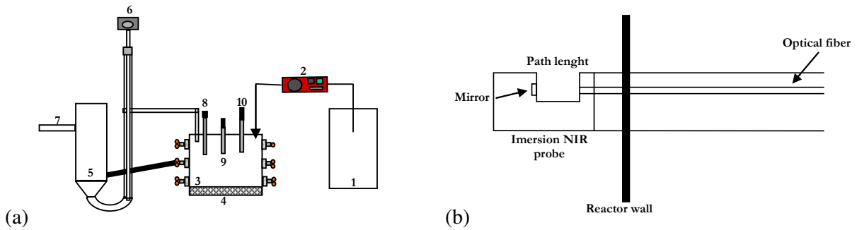
Figure 1. (a) Schematic layout of the plant: (1) effluent, (2) feeding pump, (3) aerated tank, (4) aeration system, (5) settler, (6) air pump; (7) outlet, (8) dissolved oxygen probe; (9) pH probe, (10) NIR spectrometer probe. (b) Schematic layout of the NIR transreflectance probe
