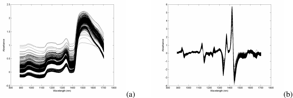
Figure 2. Raw (a) and pre-treated (b) spectra for the data collected at the aerobic reactor during a week of operation.
