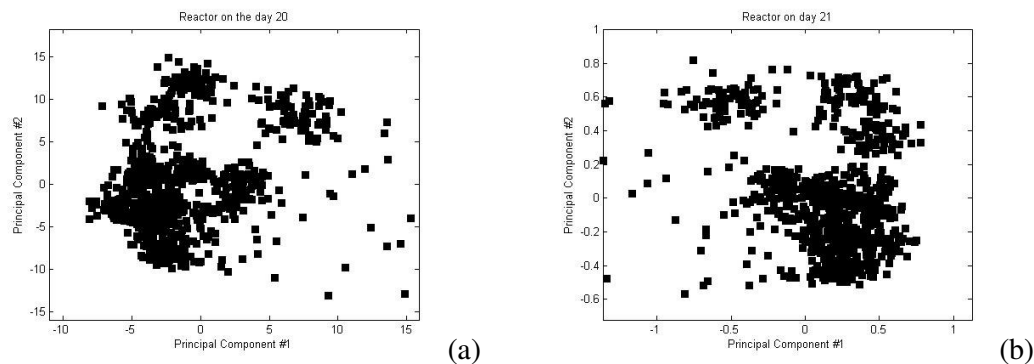
Figure 5. Score plots obtained after a continuous monitoring period with the probe immersed in the reactor for days 20 (a) and 21 (b), after the increase in the influent charge.
