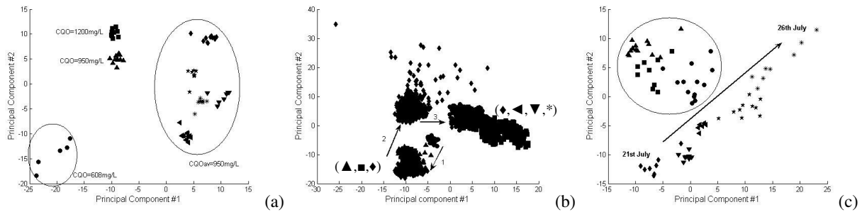
Figure 4. Score-plot of the first two principal components from the PCA model of the NIR spectra from the feed (a), reactor (b) and settler (c) sample sets. The symbols between brackets on figure b help to identify the days which are represented in each cluster.
