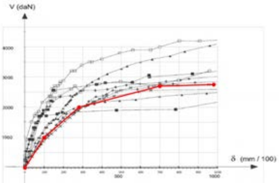
(b) Figure 4 a) Mesh with detailing, where k_x is the stiffness of the no-tension springs and k_y is the stiffness of the springs representing the shear dowels; b) Constitutive law for shear springs (red curve) with results obtained by (Giuriani 2012).
