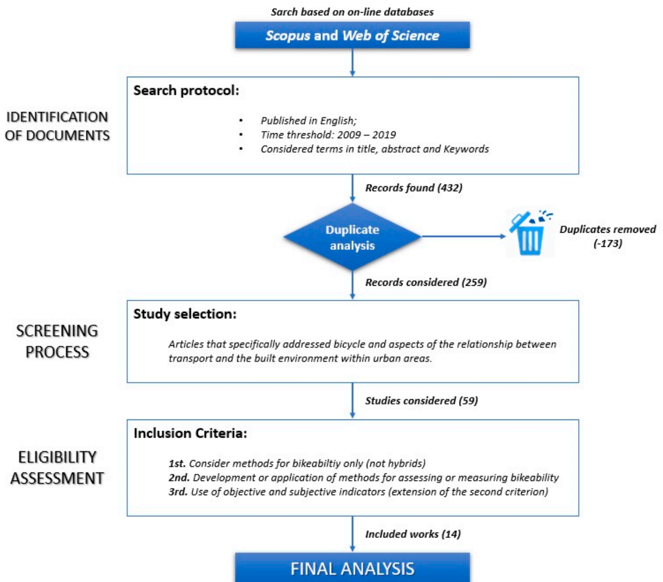
Figure 3. Methodological flowchart.
