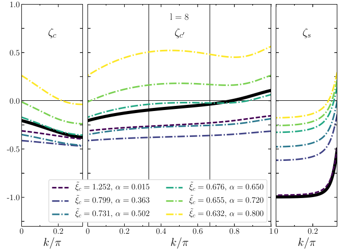
FIG. 7. The exponents that control the line shape near the MoSe 2 line defect ARPES peaks and corresponding theoretical c , c' , and s branch lines, respectively, in Fig. 6(a). They are here plotted as a function of the momentum k for u = 0.18 , n_e = 2/3 , l = 8 , and different \tilde{\xi}_c and thus \alpha values. The black solid lines refer to the conventional 1D Hubbard model ( \alpha_0 = 0.0011336 and \xi_c = 1.367 ) and the red dashed and blue (dashed-dotted and full) lines to \alpha < 1/8 and \alpha > 1/8 values, respectively. The c line, c' line, and s line whose negative exponent ranges agree with the ARPES (k, \omega) -plane peaks in Fig. 6(a) are those whose c' branch-line exponent crosses zero at k/\pi = 0 . For such lines, \tilde{\xi}_c = 0.655 , \alpha = 0.72 , and R_{\text{eff}} = 1.01 in units of lattice spacing. The \tilde{\xi}_c value below which the effects of long-range interactions become stronger is \tilde{\xi}_c^\circ = 1/\xi_c = 0.731 .
