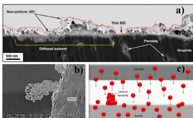
Figure 5 – Scanning electron microscopy (SEM) image of the SEI layer in a LIB anode 54 a) SEM image of a lithium dendrite 55 (b); schematic representation of the lithium dendrite formation process (c).
