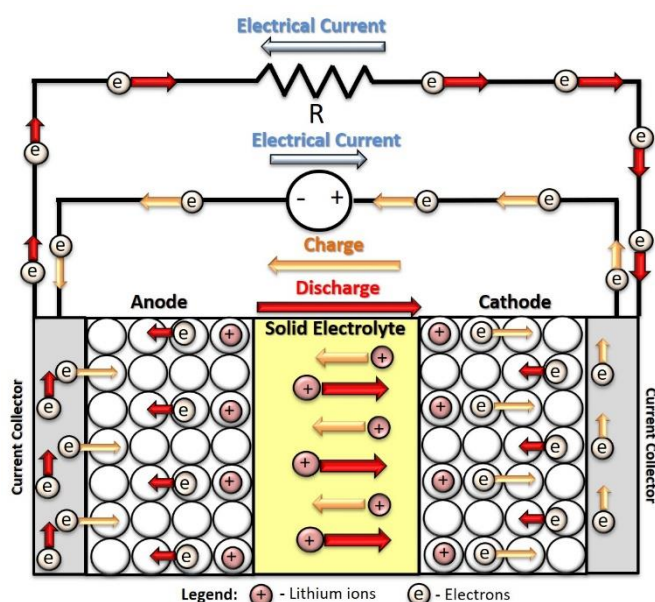
Figure 1 – Schematic representation of the composition and charge/discharge process of an archetypal LIB.
