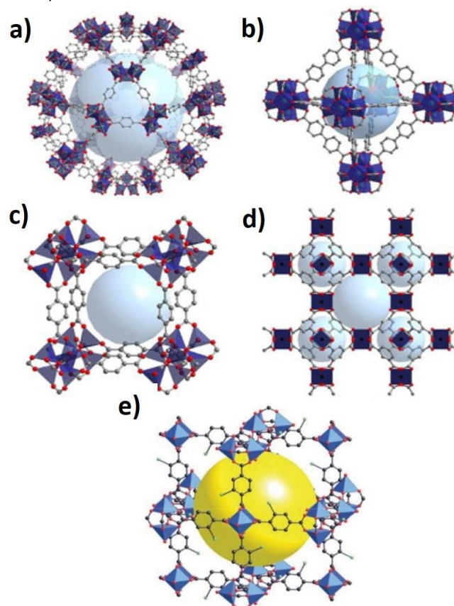
Figure 9 – Typical structure of representative MOFs: MIL-101 (a), UIO-67 (b) MOF-5 (c), HKUST-1 (d) 125 and MOF-101 (e) 126, 127 .
