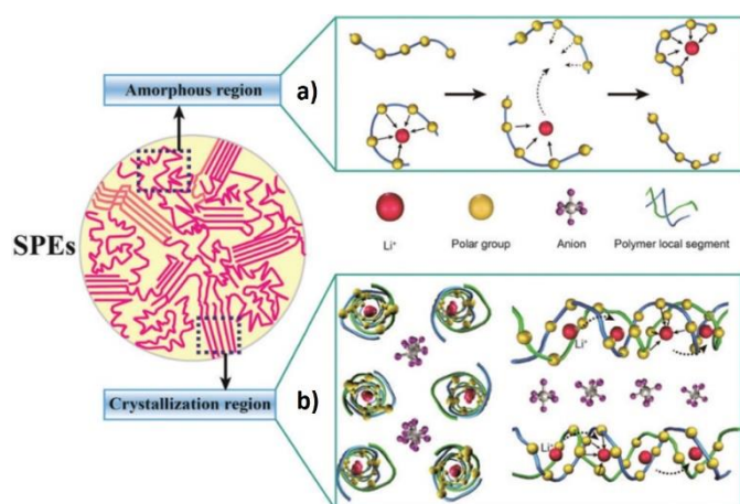
Figure 6 – Schematic illustration of conduction mechanisms in amorphous (a) and crystalline (b) SPEs 66 .
