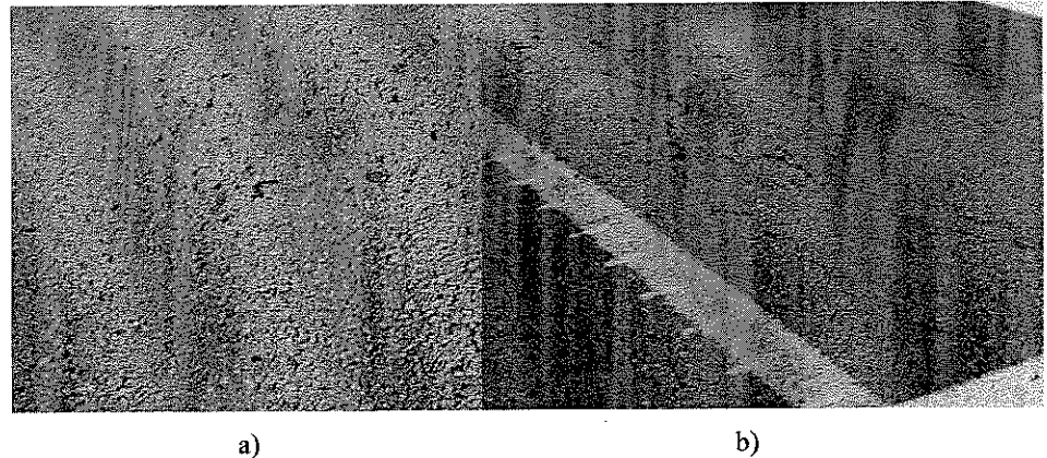
Figure 3. Distresses on EN 206 VARIANT: a) ravelling; b) cracking
