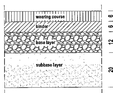
Figure2. Pavement structure
