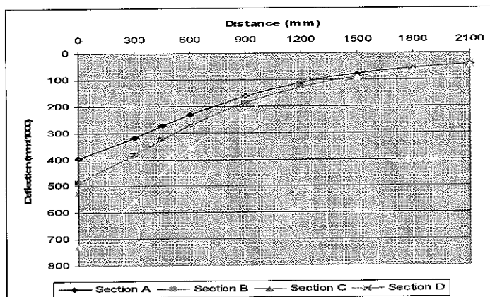
Figure 4 - Representative deflection bowls for each road section
