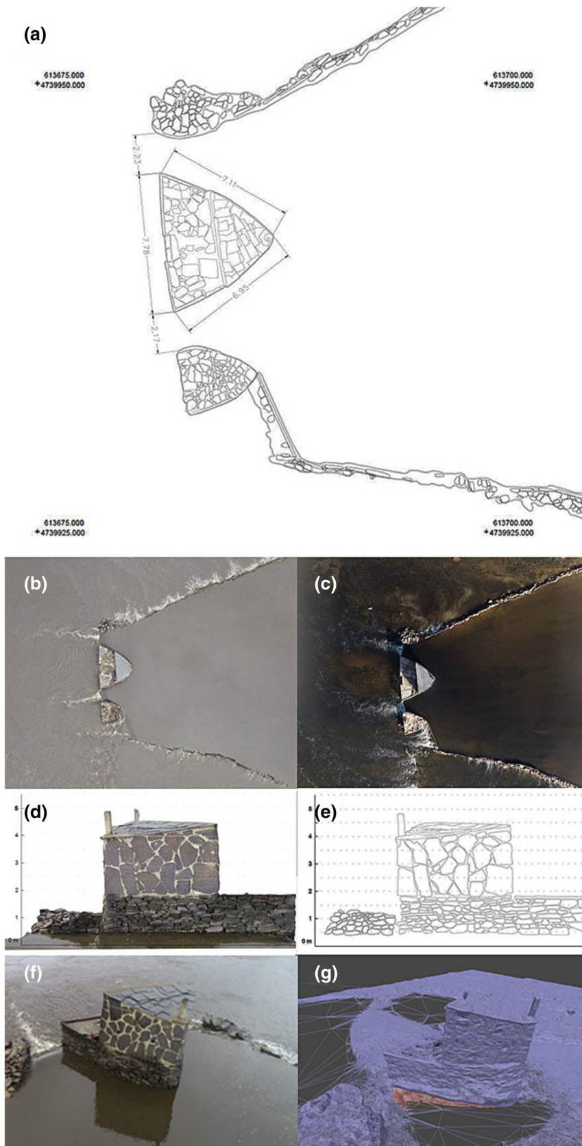
FIGURE 12 (a) Fishery planimetric digitalization. (b) Detailed orthophoto obtained on a cloudy day. (c) Detailed orthophoto obtained on a sunny day. (d) Orthophoto of the side view of a weir. (e) Planimetric digitalization of the side view. (f) Photo with reflection. (g) Duplication in the mesh. [Colour figure can be viewed at wileyonlinelibrary.com ]
