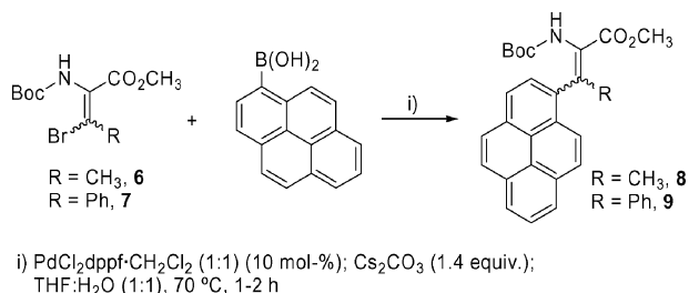
Scheme 3. Synthesis of the methyl esters of N -( tert -butoxycarbonyl)- \beta -(pyren-1-yl)dehydroamino acids.
