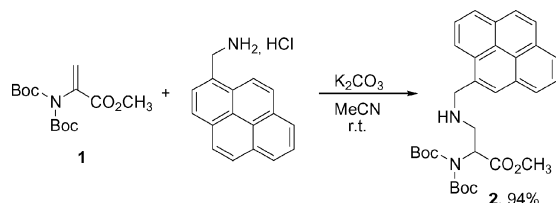
Scheme 1. Synthesis of the methyl ester of N,N -bis( tert -butoxycarbonyl)- \beta -[(pyren-1-yl)methylamino]alanine.
