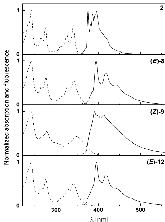
Figure 1. Normalized absorption (dashed lines) and fluorescence (solid lines) ( \lambda_{\text{exc}} = 342 \text{ nm} ) spectra of compounds 2 , ( E )- 8 , ( Z )- 9 and ( E )- 12 in cyclohexane (concentrations are 2 \times 10^{-5} \text{ M} for absorption and 3 \times 10^{-6} \text{ M} for emission).
