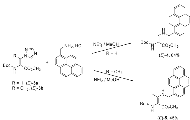
Scheme 2. Synthesis of the E isomer of the methyl esters of N -( tert -butoxycarbonyl)- \beta -[(pyren-1-yl)methylamino]dehydroamino acids.
