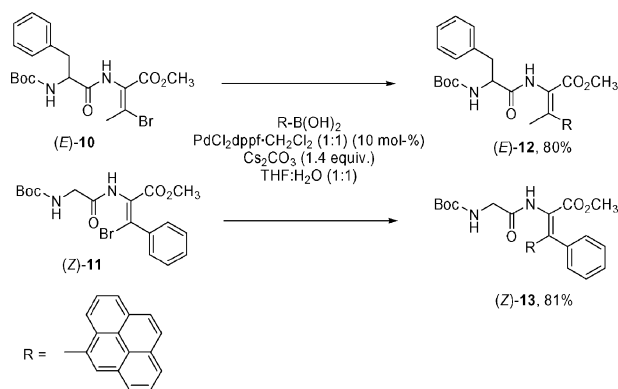
Scheme 4. Synthesis of the methyl esters of N -( tert -butoxycarbonyl)- \beta -(pyren-1-yl)dehydrodipeptides.
