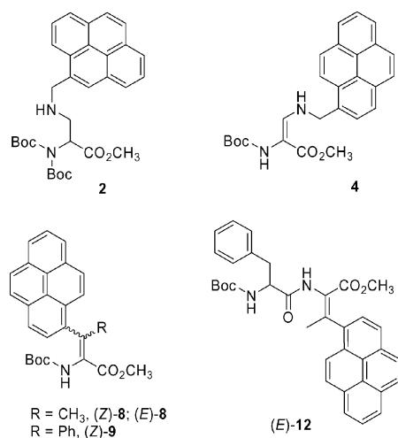
Scheme 5. \beta -(Pyrenyl)amino acid derivatives submitted to cyclic voltammetry and photophysical studies.
