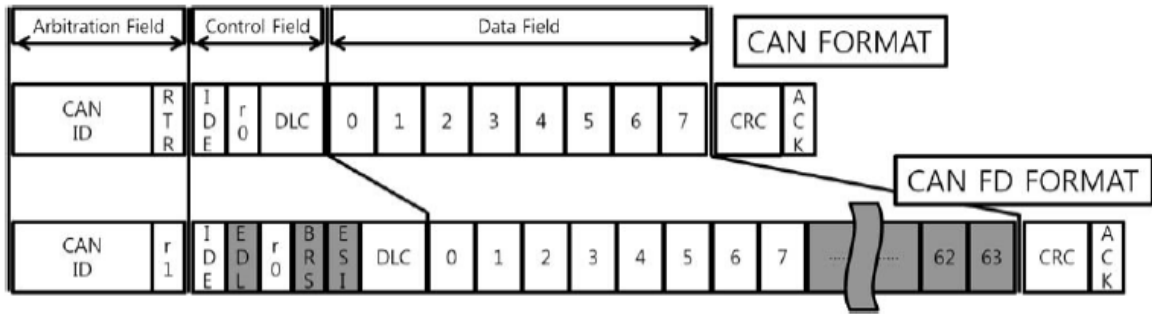
Figure 9: Comparison of CAN and CAN FD data frames (Woo et al., 2016)
