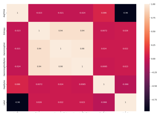
Figure 28: Correlation between extracted features obtained from the Automotive Controller Area Network (CAN) Bus Intrusion Dataset v2
