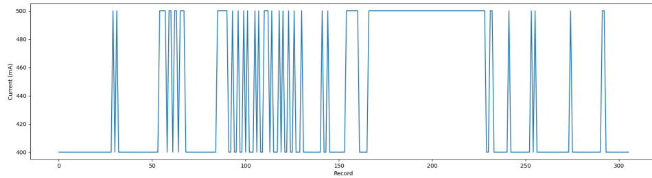
Figure 21: Power consumption from the Raspberry Pi while executing the proposed IDS
