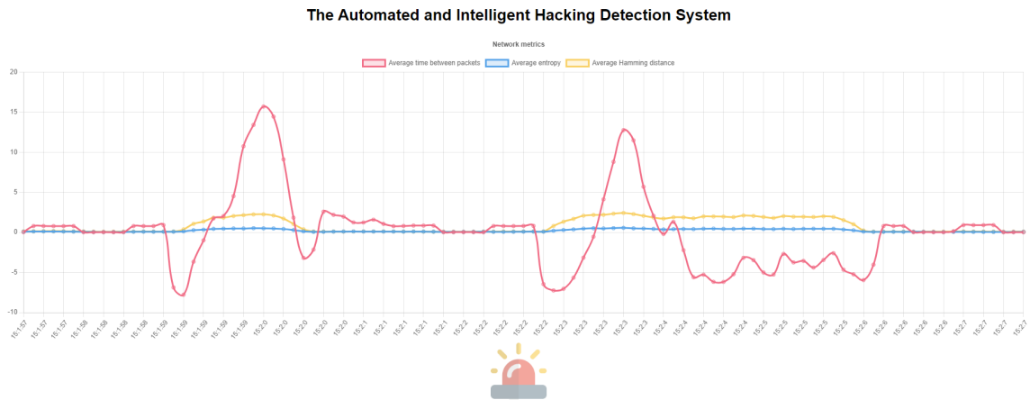
Figure 22: Graphical interface
