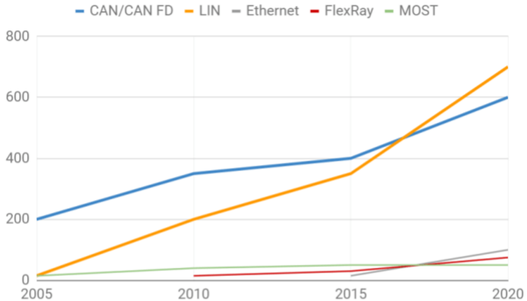
Figure 5: Number of nodes in automotive by technology (CSS Electronics, 2021)
