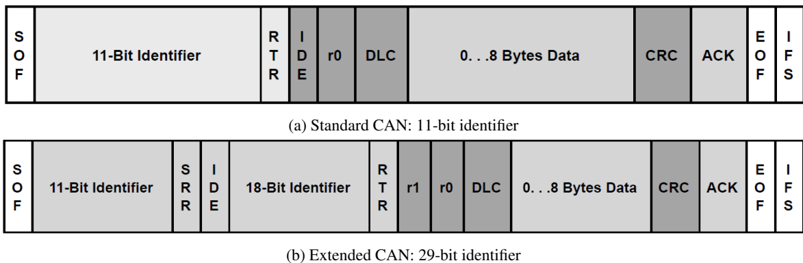
Figure 8: Classical CAN frame structure (Corrigan, 2002)
