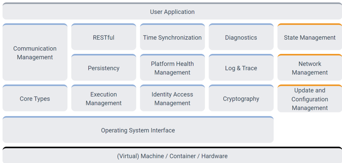
Figure 3: The AUTOSAR Adaptive Platform architecture (AUTOSAR)
