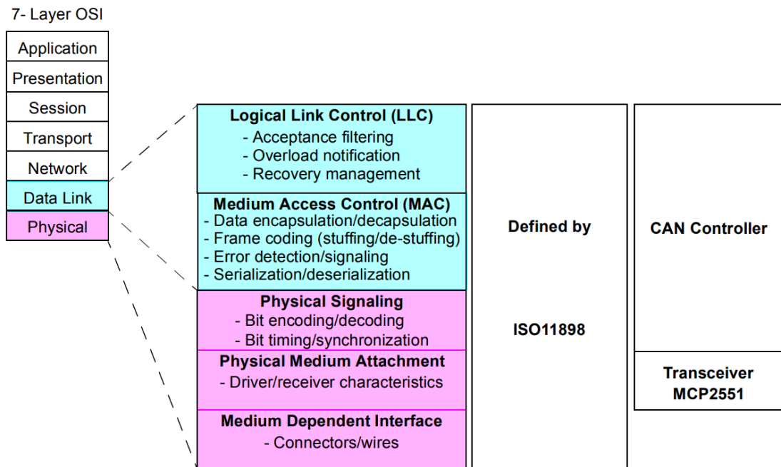
Figure 6: CAN and the OSI model (Richards, 2002)
