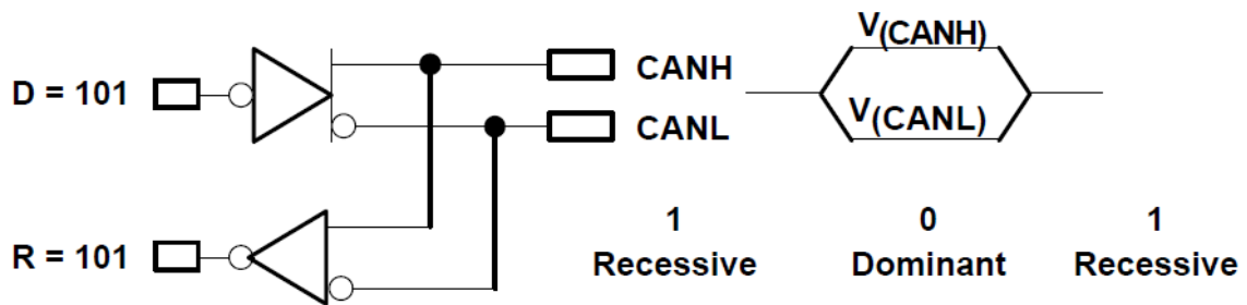
Figure 7: The inverted logic of a CAN bus (Corrigan, 2002)
