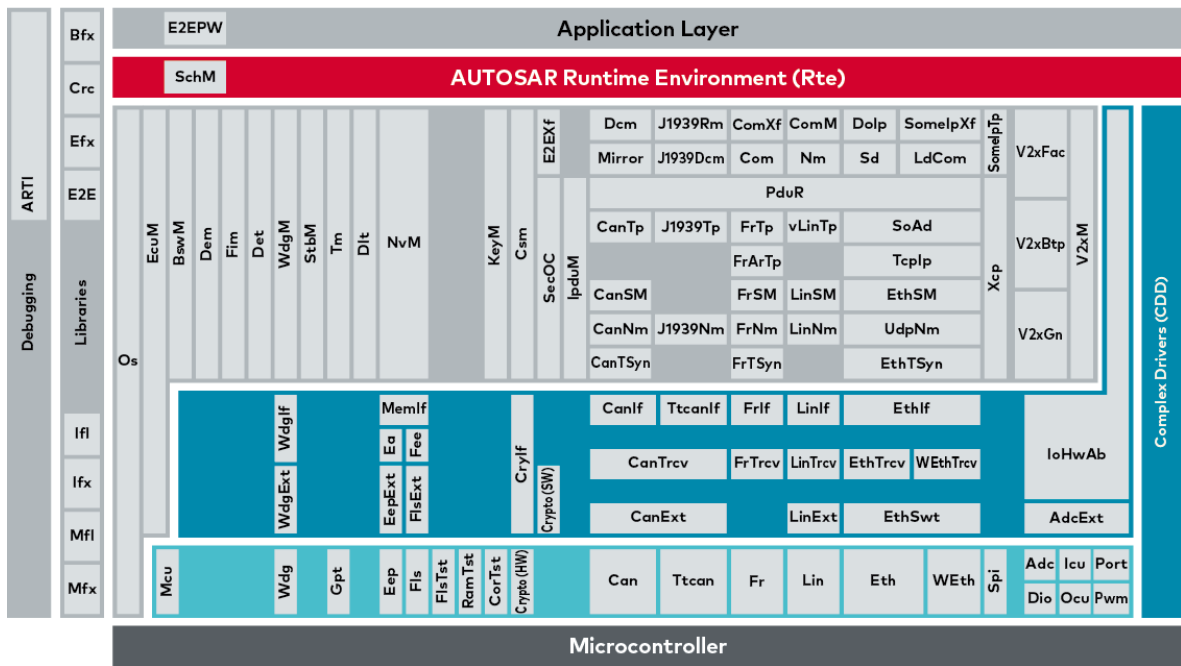
Figure 2: The AUTOSAR architecture (Vector)
