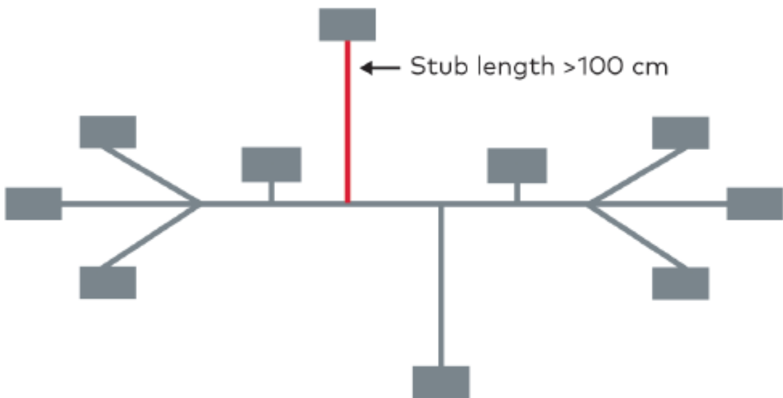
Figure 12: Comparison between 10BASE-T1s and CAN XL topology requirements (Garnatz and Decker, 2020)
