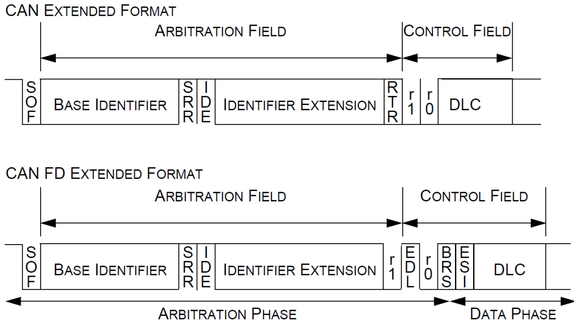
Figure 11: Comparison of extended CAN and CAN FD data frames (Bosch, 2012)
