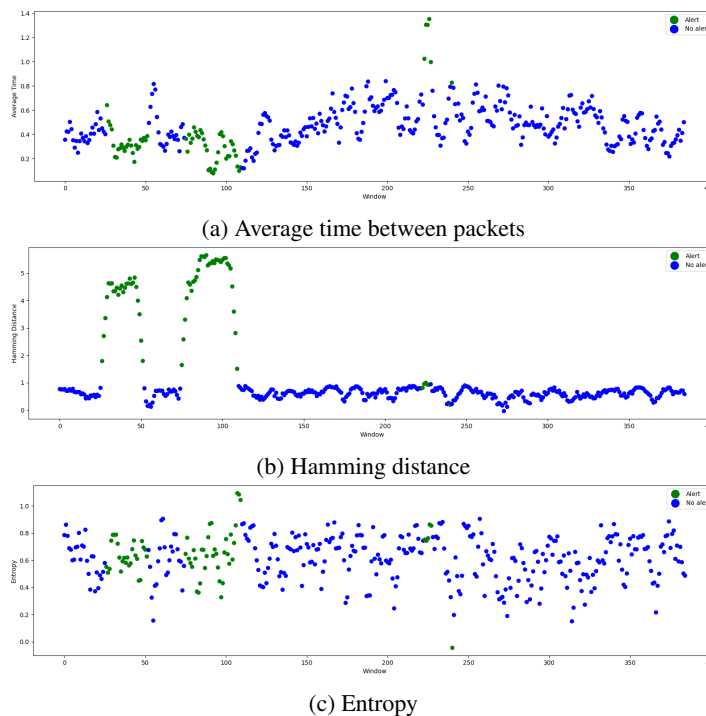
Figure 24: Features extracted from the spoofing attack present in the custom dataset
