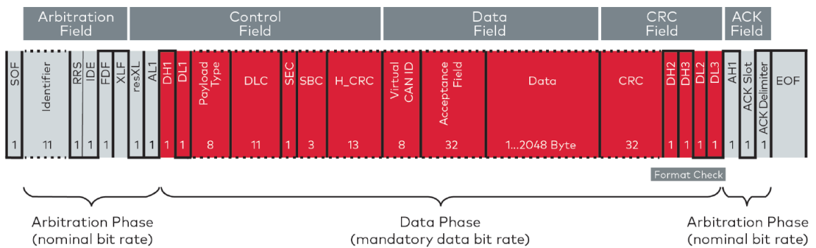
Figure 13: Current status of development of the CAN XL frame (Garnatz and Decker, 2020)
