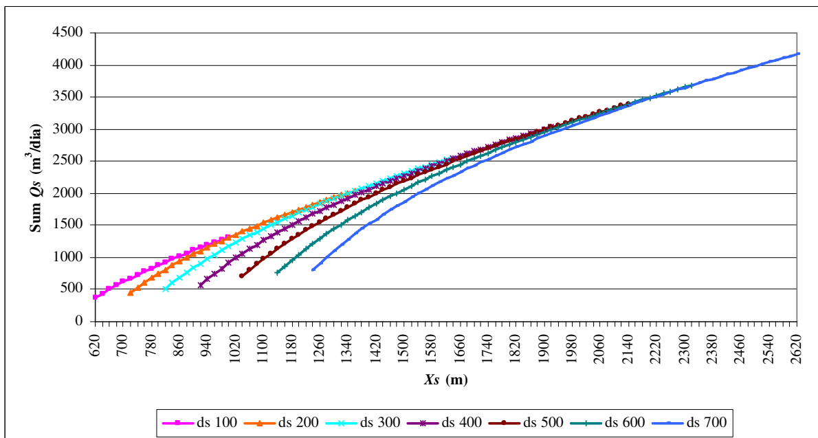
Fig. 6. Extractions for 3 wells versus location X_s and security distance ds = 100, 200, \dots, 700 m
