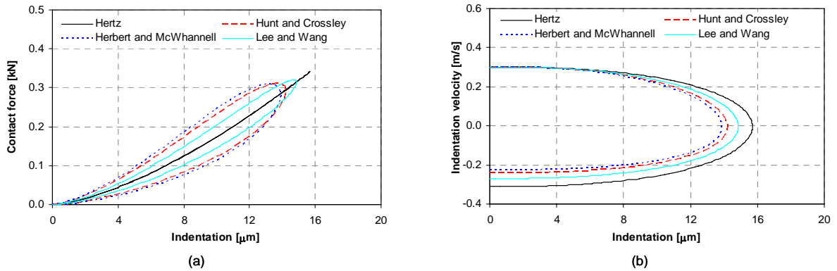
Fig. 5 Externally colliding spheres modeled by Hertz, Hunt and Crossley, Herbert and McWhannell, and Lee and Wang contact force models: (a) Force-indentation relation; (b) Phase portrait.
