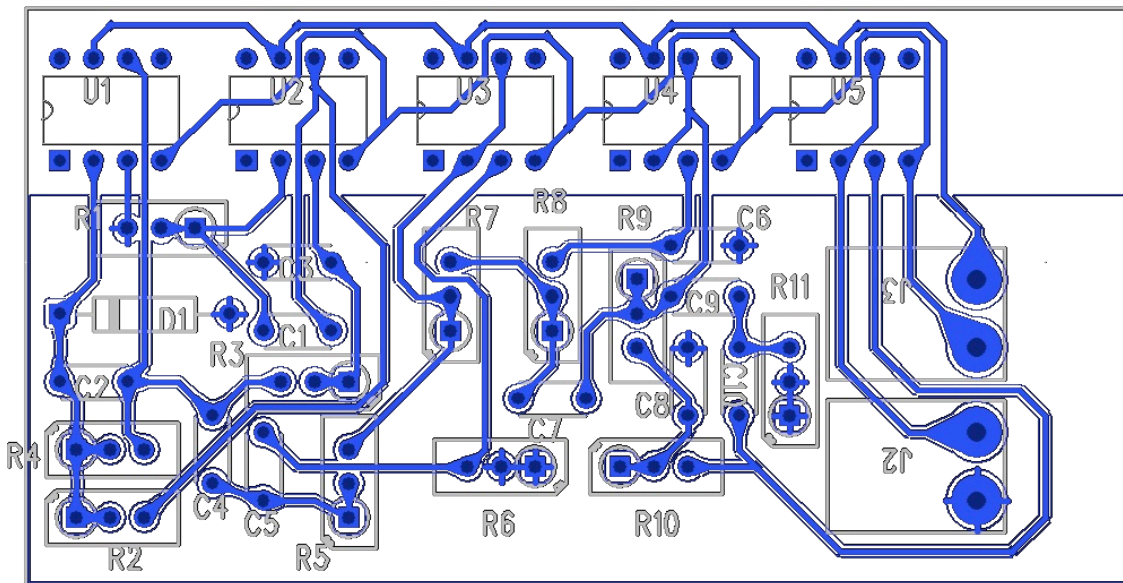
Figure I.2 OE system PCB layout.
