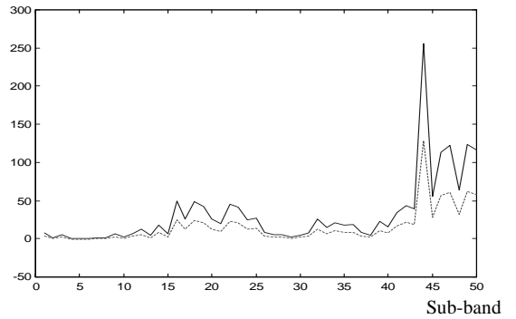
Figure 2. Relative deviation caused by additive white noise at 0 dB at the beginning of digit “zero” when working in the power spectral density domain (normal line) and in the power spectrum density normalisation domain (dashed line).
