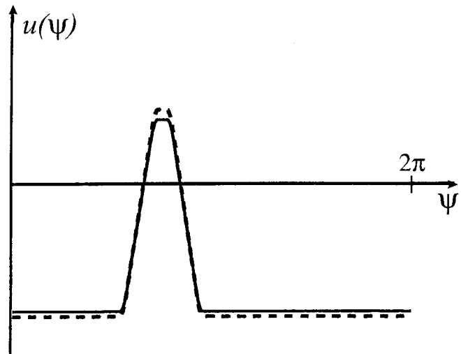
Fig. 7. A localized positive peak of activation (dashed line) is stable in the presence of input. It remains stable if input is removed (solid line). The peak is sustained by local self-excitation. Its lateral diffusion is limited by global inhibition. This is the memory mechanism in the dynamic field. The position of the peak within the field is marginally stable, however, so that the contents of memory may slowly degrade with time.
