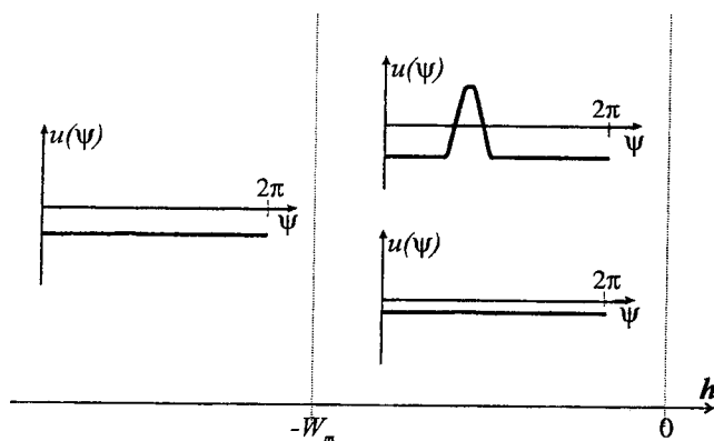
Fig. 8. The different stable states of the field dynamics without input are illustrated as a function of the resting level, h . Below a critical level of h ( -W_m ), only the homogeneous "off" state of the field is stable. All sites have the same negative level of activation. Above the critical level (but still below zero), two types of stable states coexist. The homogeneous state persists, but a positive localized peak of activation is likewise stable (irrespective of where it is positioned). This bistable regime serves the memory function, while the monostable regime induces forgetting or resetting of memory. Memory peaks are set by applying sufficiently strong input (see detection mechanism).
