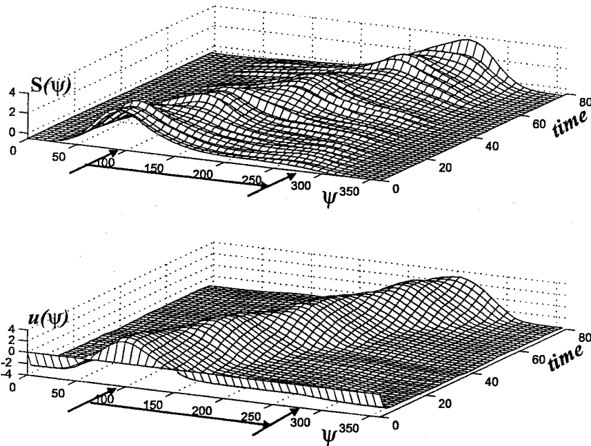
Fig. 15. The robot was positioned with an orientation of 180 deg with respect to the external axis. The sound source was moved continuously from an initial direction of 90 deg (indicated by the left arrow) all the way to 270 deg (indicated by the right arrow). Top: sensory information is monomodal and its maximal location varies continuously. Bottom: the field evolves a peak of positive activation that tracks and follows the moving input peak.
