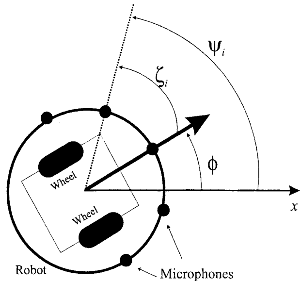
Fig. 10. Sensory information about sound targets is acquired by five microphones, each pointing into a direction \zeta_i ( = -90, -45, 0, 45, 90 deg), with respect to the heading direction, \phi , of the robot. The direction in the world at which microphone i is pointing is \psi_i = \phi + \zeta_i .
