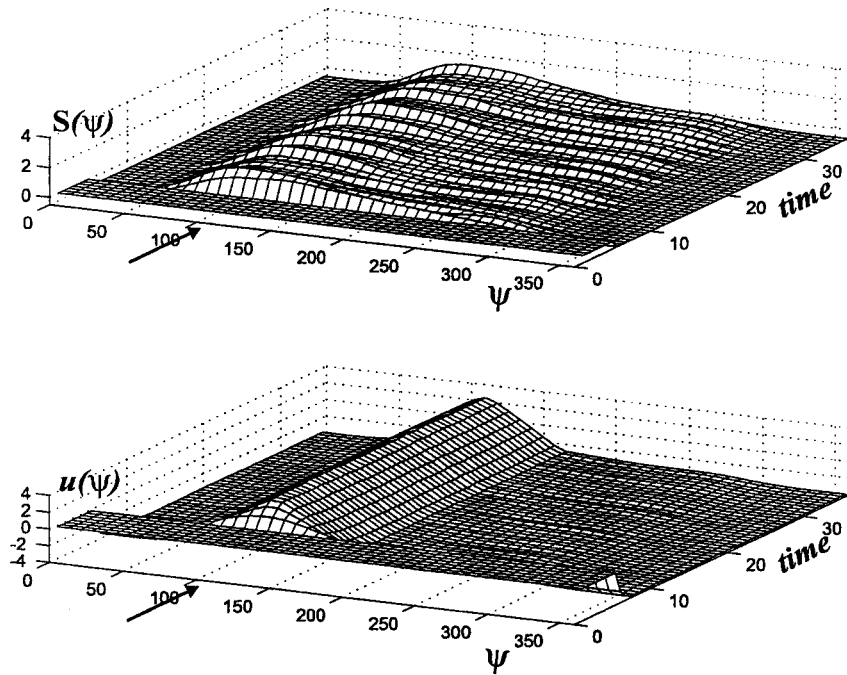
Fig. 13. A sound source was placed at an angular position of 112.5 deg (the location indicated by the arrow) with respect to the world axis. Robot orientation was 180 deg; the five microphones were thus pointing in the directions 90, 135, 180, 225, and 270 deg. Top: sensory information leads to a broad monomodal input distribution. Bottom: the field activation relaxes to a stable localized peak centered over the maximum of the input. The estimated sound orientation is 115 deg.
