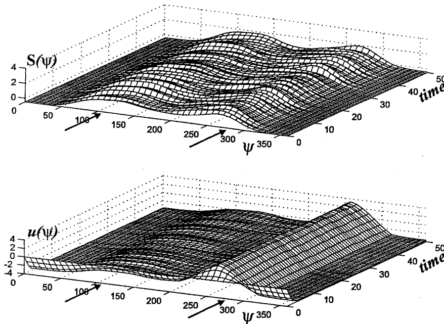
Fig. 16. The robot was placed with a heading direction of 180 deg with respect to the external axis. Two sound sources, the pulse modulated wave and the harmonic wave, were placed at angular positions 112.5 deg and 270 deg (as indicated by the arrows), respectively. Top: under such experimental setup, the sensory input to the field is bimodal. Bottom: competition takes place and as a result the field makes a decision. The field evolves a single peak of positive activation centered near the input peak located at 270 deg. Thus, the left target is selected.
