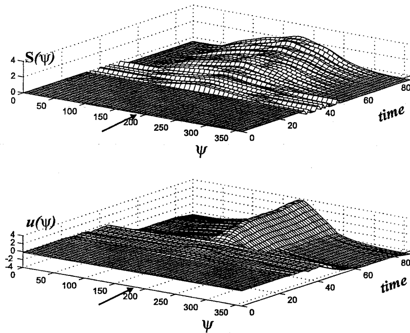
Fig. 12. Here, the target detection behavior of the field is shown. Direction is in degrees (deg) and time in seconds (sec). The sound source was placed in the forward direction of the robot (indicated by the arrow), and sound intensity was increased from 0 to 2.5. Robot position and orientation (180 deg with respect to the world axis) in space was kept fix. Top: the input to the field, S(\psi) , is monomodal and its strength increases in time. Bottom: while the input is weak, the field is in the state in which it is all off and thus no target is detected. At time t \approx 55 sec, the input strength is sufficiently strong to trigger the detection of the sound source. From this point on, the stable state of the field is a localized peak of positive activation centered over the location of maximal input.
