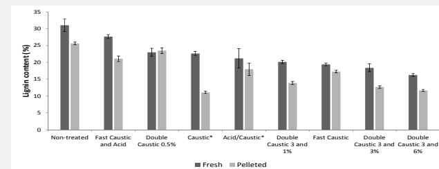
Figure 2 – Lignin composition of 100 g dried carrier for each treatment. * Methods performed according to Brányik et al. (2001).
