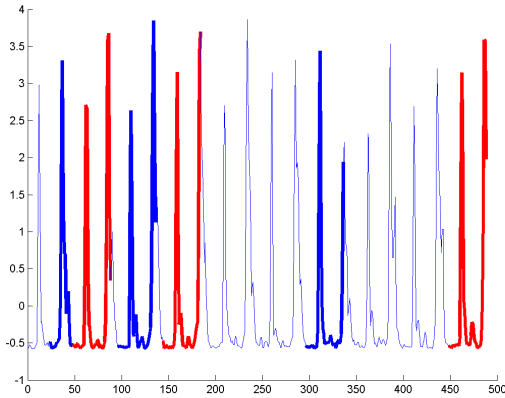
Figure 6: Motif 15 shown in thicker line (alternating blue and red) overimposed on the original time series (x-Time/y-Amplitude).
