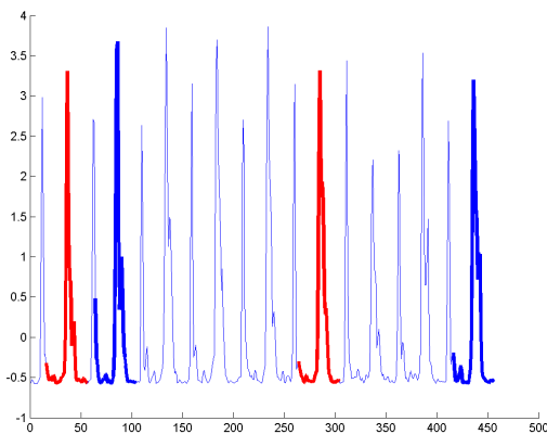
Figure 7: Motif 0 shown in thicker line (alternating blue and red) overimposed on the original time series (x-Time/y-Amplitude).
