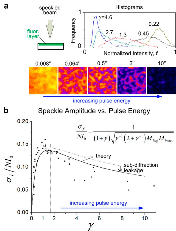
Figure 3. Optimal speckle generation. (a) In a uniform fluorescent layer, increasing \gamma leads initially to a spreading of the histogram, resulting in increasingly visible speckles. For \gamma \gg 1 , the tendency is reversed, ultimately driving all fluorophores toward the bleached state. Labels in the bottom row correspond to laser exposure time in seconds. (b) Experimental data for the dependence of speckle amplitude on \gamma , obtained by performing the experiment outlined in a. Dashed curve corresponds to fitting of the model curve (Eq. 3) using the theoretically calculated baseline for the loss of contrast factor caused by imaging, M_{img} = 2.12 , and the instrumental factor, M_{instr.} , which arises as the single-fitting parameter in the model. Both the shape and the peak position are intrinsic to the model and not dependent on fitting. The solid curve applies a \gamma -dependent correction to M_{img} , as obtained by computer simulation to correct for subdiffraction leakage, which becomes relevant for \gamma \gg 1 (Fig. S4 d and Materials and methods).
