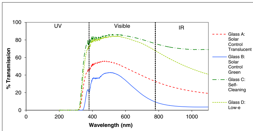
Fig. 5. Transmission curves.
