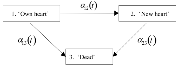
Figure 1. Illness-death model for Transplant Heart Data.
