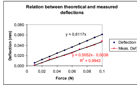
Fig. 12. Relation of theory and practical deflections. In blue the theoretical expression, and in red the measured deflection
