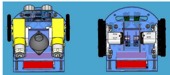
Figure 4: Final design of the Traction System in the Beta version of Kid Grigora Rookie and Semi-Pro.
