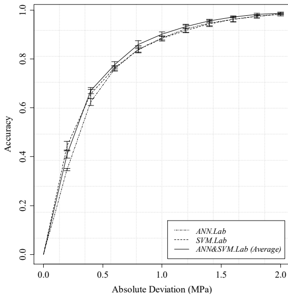
Figure 2. Comparison of ANN.Lab, SVM.Lab, and ANN&SVM.Lab performance in q_u prediction of laboratory soil-cement mixtures based on REC curves.
