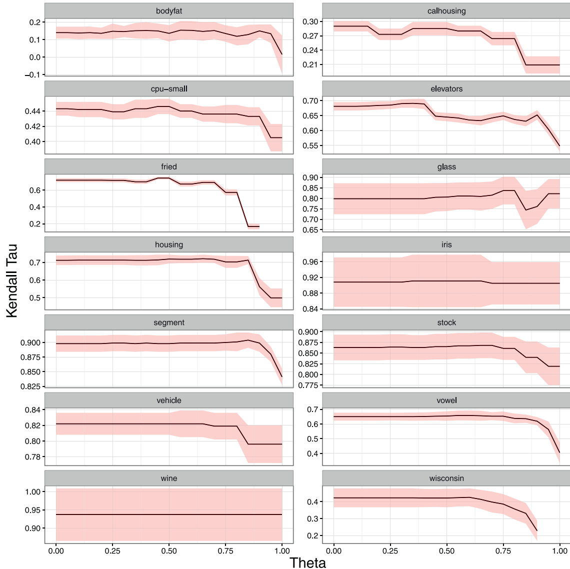
Fig. 1. Average accuracy (Kendall \tau ) of CAREN as the value \theta varies. (The shaded area represents the standard deviation).
