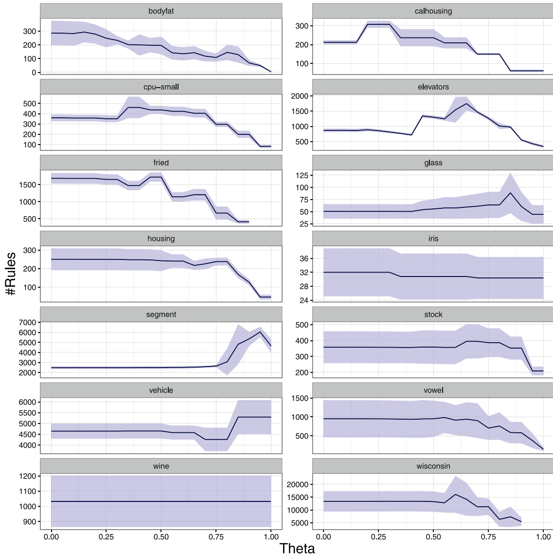
Fig. 3. Number of Label Ranking Association Rules generated by CAREN as the value \theta varies. (The shaded area represents the standard deviation).
