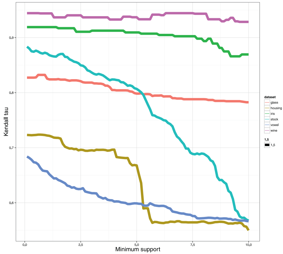
Fig. 5. Average accuracy (Kendall \tau ) of CAREN as the value minsup varies.
