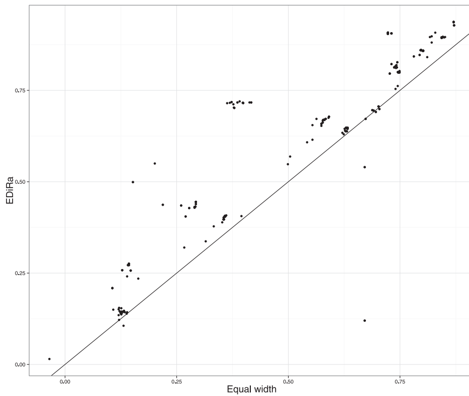
Fig. 6. Ranking accuracy (Kendall \tau ) of CAREN after the discretization of data using equal width and EDiRa . This plot aggregates all the experiments carried out for each dataset, which means that each dataset is represented multiple times, with different parameter settings.
