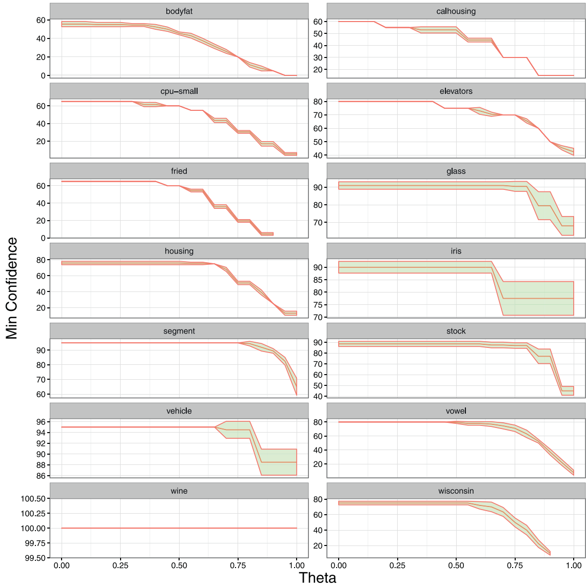
Fig. 4. Minimum confidence as the value \theta varies. (The shaded area represents the standard deviation).
