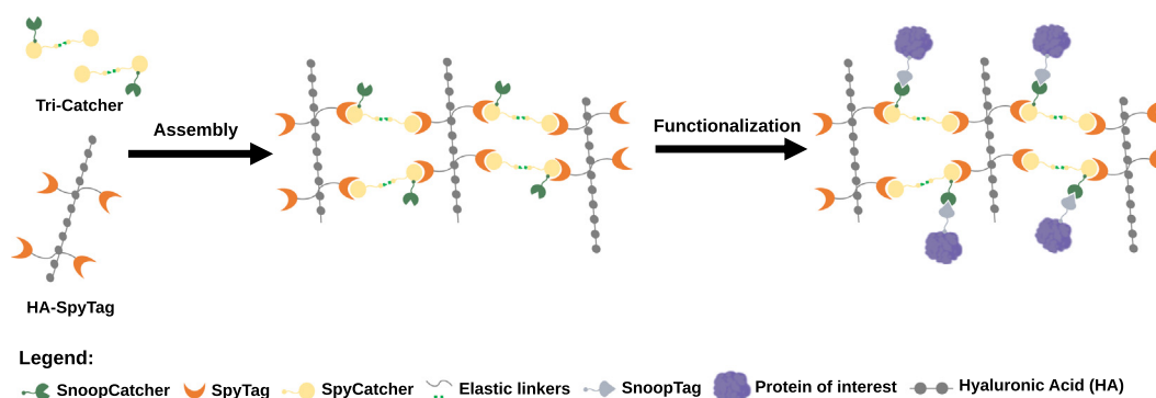
Fig. 4. Exploration of the Tag/Catcher system properties for the self-assembly and functionalization of engineered protein-based hydrogels. By coupling HA-SpyTag (HA coupled to two SpyTags linked by an elastin-like polypeptide) with TriCatcher (two SpyCatcher linked by an elastin-like polypeptide with/without an RGDSP integrin-binding site and a C-terminal SnoopCatcher), Wieduwild and Howarth [89] rapidly assembled stable hyaluronan hydrogels via SpyTag/SpyCatcher isopeptide bond formation. Functionalization was further achieved by linking SnoopTagged-proteins to the SnoopCatcher without interfering with the hydrogels' mechanical behavior.
