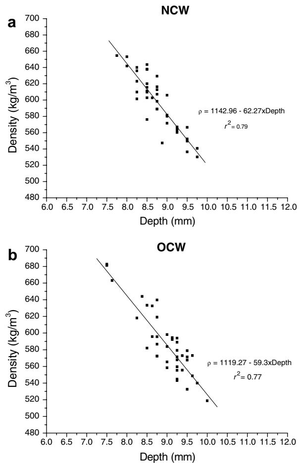
Fig. 6. Relation between pin depth (Pilodyn) and density: (a) NCW group and (b) OCW group.
